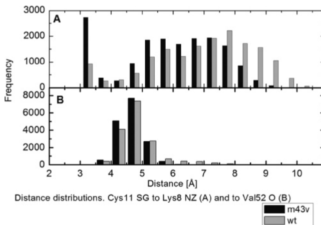
FIGURE 7: Distance distributions Cys11 S\gamma to Lys8 N^{\zeta} and Val52 O in glutaredoxin 3 Met43Val mutant and wild-type simulations. Panel A shows the shorter average distances between Cys11 S\gamma and Lys8 N^{\zeta} as well as the narrower distance distribution in glutaredoxin 3 Met43Val. Panel B shows the slightly shorter average distances between Cys S\gamma and Val O in glutaredoxin 3 Met43Val.
