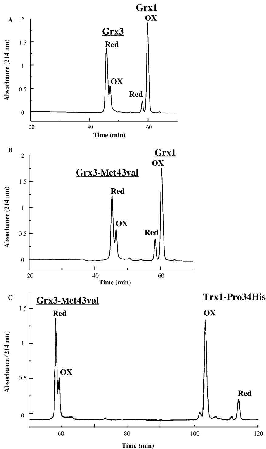
FIGURE 4: Reverse-phase HPLC chromatograms of redox equilibria between different glutaredoxin and thioredoxin species. Equal concentrations ( 50 \mu\text{M} ) of reduced His 6 -tagged E. coli glutaredoxin 3 or glutaredoxin 3 M43V were incubated with either oxidized glutaredoxin 1 or thioredoxin 1 P34H in potassium phosphate pH 7.0, 1 mM EDTA buffer for 12 h at 25 °C, followed by acid quenching to pH 2.5 before separation of the different species on a C 8 reverse-phase HPLC column (see Experimental Procedures for details). (A) Glutaredoxin 1 and glutaredoxin 3. (B) Glutaredoxin 1 and glutaredoxin 3 M43V. (C) Thioredoxin 1 P34H and glutaredoxin 3 M43V.
