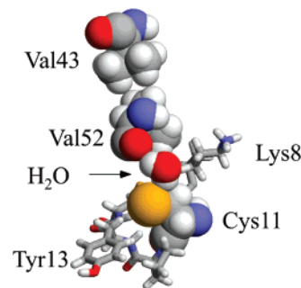
FIGURE 6: Snapshot from simulation of the glutaredoxin 3 M43V mutant. A water molecule in bridging position between Val52 O and Cys11 S\gamma is shown. The structure shows Lys8, which at this time is turned away from Cys11, and residue 43 (valine), which makes stable hydrophobic contact with valine 52.
