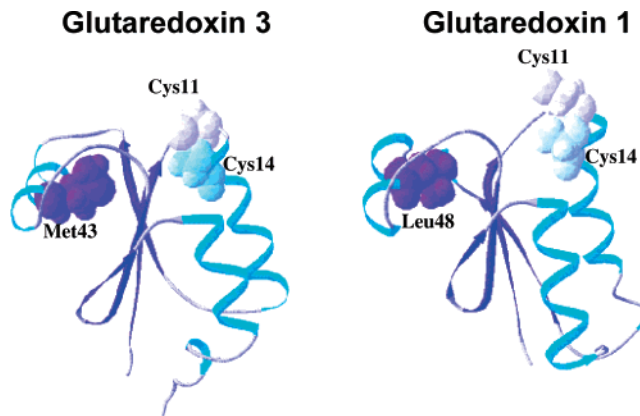
FIGURE 1: Structures of glutaredoxin 1 and 3. E. coli glutaredoxin 1 (Grx1, PDB file 1GRX) (right) and glutaredoxin 3 (Grx3, PDB file 3GRX) (left) consist of the core thioredoxin fold. The two structures are viewed from identical orientation. Secondary structures \alpha -helix and \beta strands are indicated. The mutated methionine 43 in Grx3 and the equivalent leucine 48 in Grx1, as well as the active-site cysteines (Cys11 and Cys14) located at the beginning of \alpha -helix 1 are presented in a space-filling model. Both structures were determined by using Ser11-X-X-Cys14 mutant proteins.
