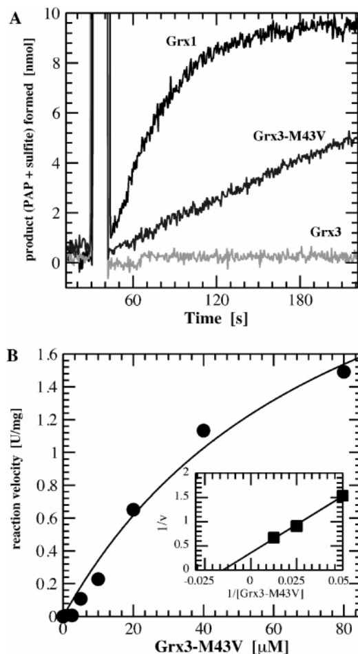
FIGURE 3: Glutaredoxin 3 Met43Val as hydrogen donor of 3'-phosphoadenylylsulfate (PAPS) reductase. PAPS reductase was measured following NADPH consumption in a coupled assay with yeast glutathione reductase as outlined in Experimental Procedures. (A) Reduction of 10 nmol of PAPS by PAPS reductase (0.5 \mu\text{g}/\text{mL} ) with glutaredoxin 1, glutaredoxin 3, or glutaredoxin 3 Met43Val as electron donors. (B) Michaelis–Menten and Lineweaver Burk plots of the initial velocity kinetics of PAPS reductase with glutaredoxin 3 Met43Val as electron donor.
